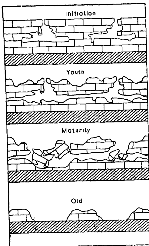
Fig. 96—The Cycle of Karst Erosion
