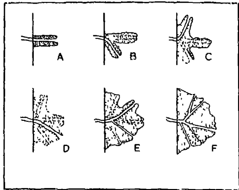
Fig. 37. Stages in formation of a Simple Delta
