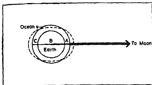
Fig. 109. Formation of Tide
