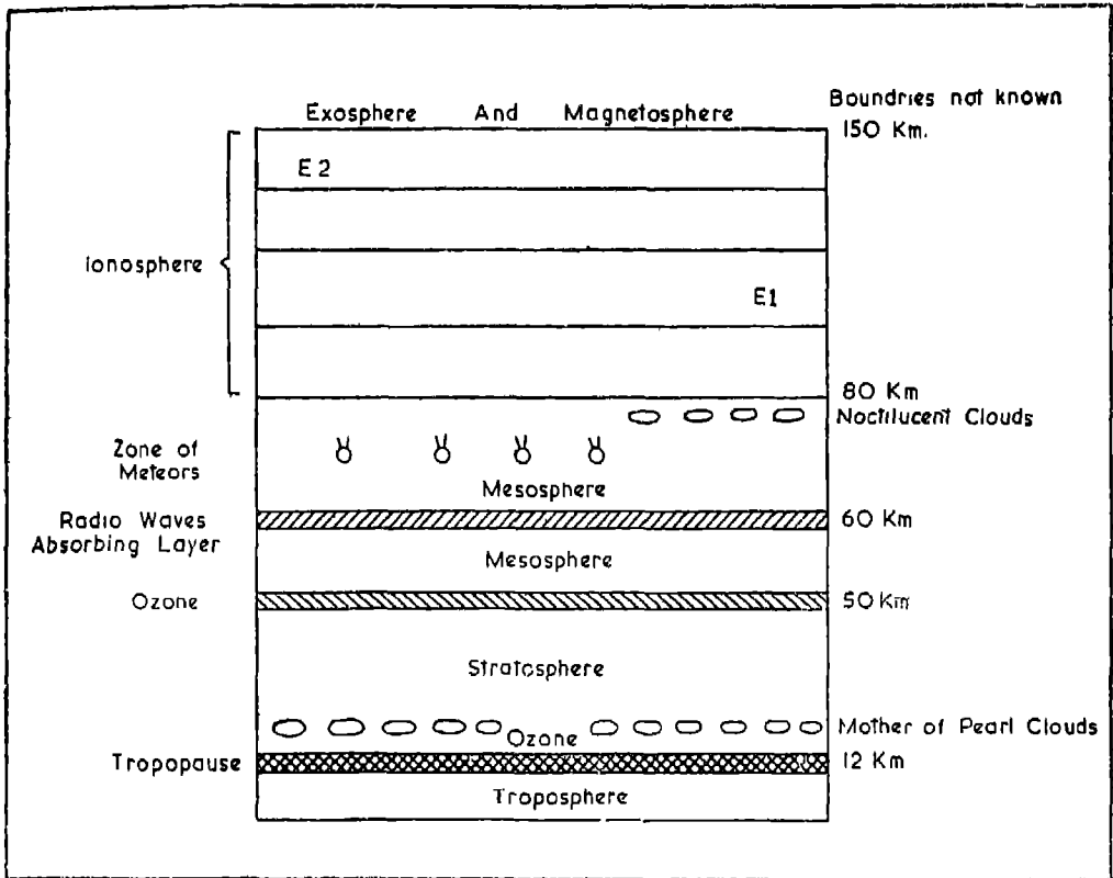
Fig. 56. Layered structure of Atmosphere
