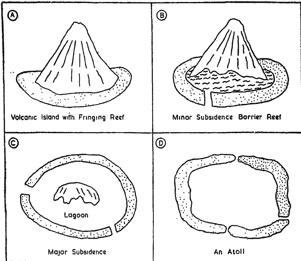
Fig. 112. Types of Reefs
