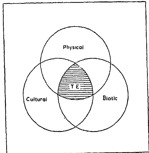
Fig. 4. Total Environment
