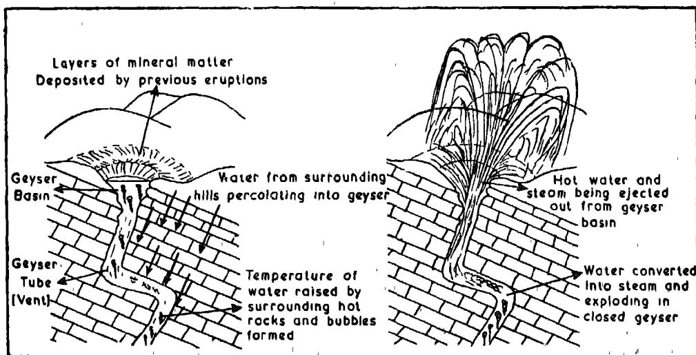
Fig. 94. Formation of Geyset
