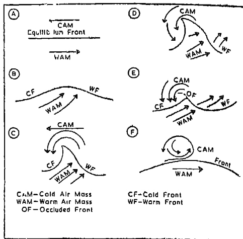
Fig. 77. Cold and Warm Air masses and Fronts
