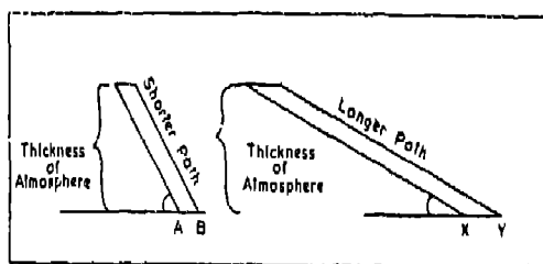
Fig. 58. Angle of incidence of insolation and Area Affected
