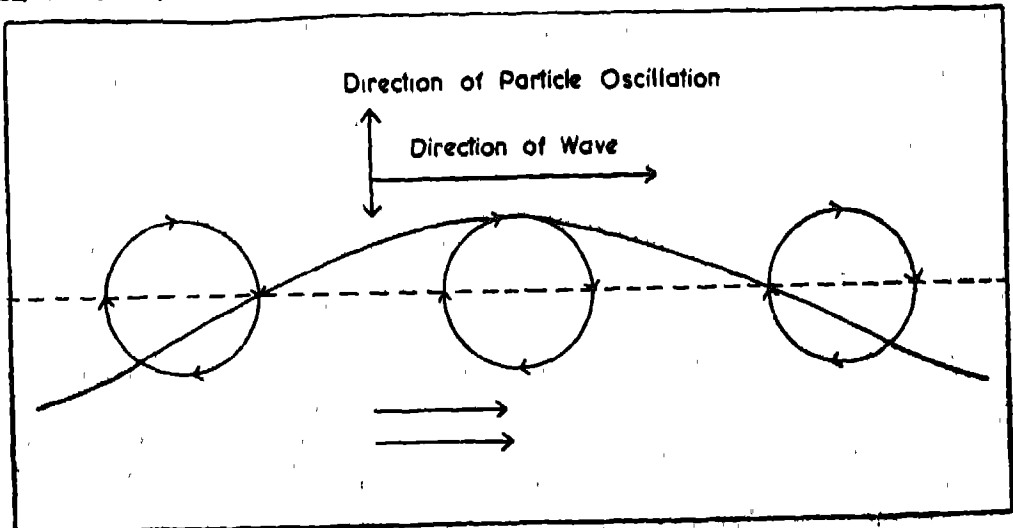
Fig. 107. Transverse Wave
