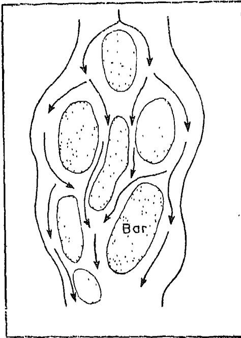
Fig. 36. Braided Stream
