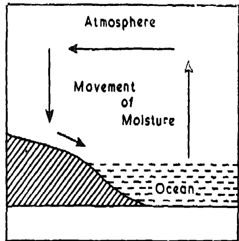
Fig. 82. Simple Hydrologic Cycle
