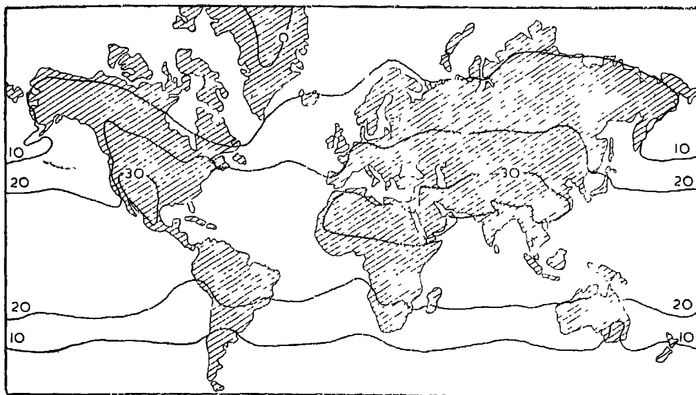
Fig. 64. July Isotherms
