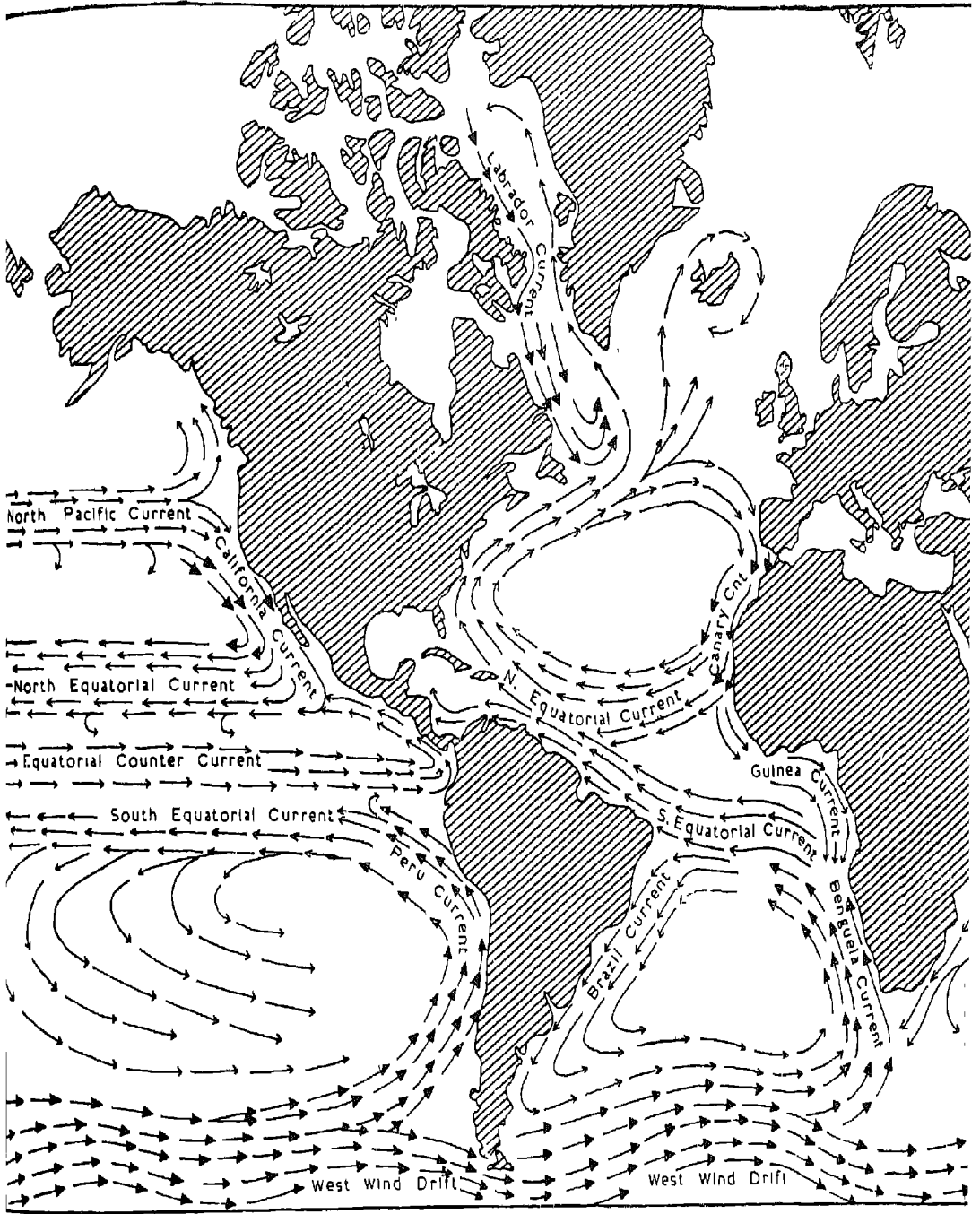
Fig 108. Ocean Currents
