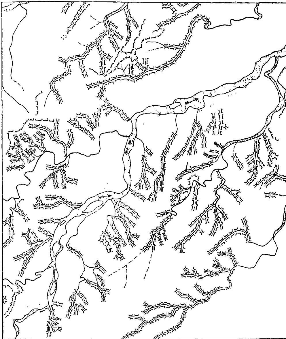
Fig. 20. Clay Topography
