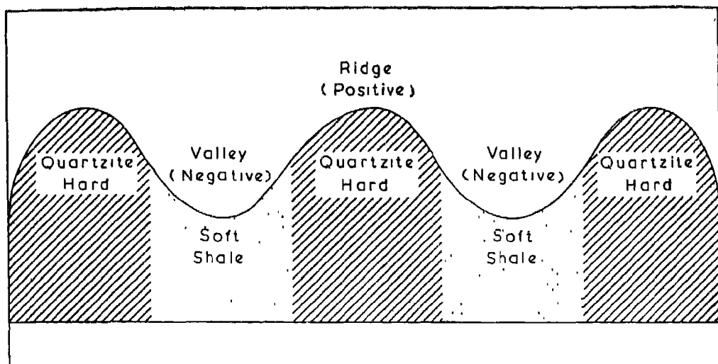
Fig. 19. Rock Hardness and Relief Features
