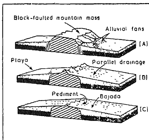
Fig. 40. The Erosional Evolution of a Pediment
