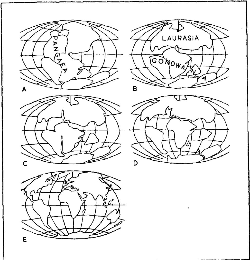
Fig. 52. Continental Drift
