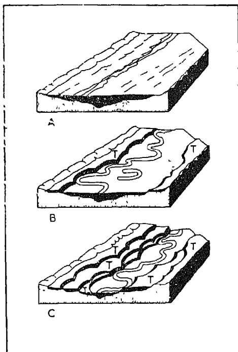
Fig. 34. Alluvial Terraces
