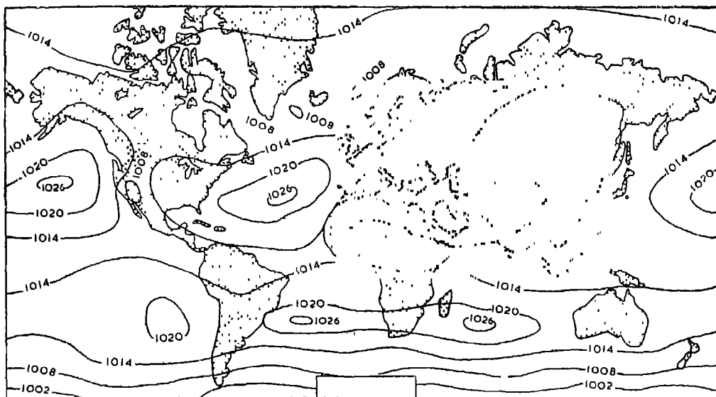
Fig. 67. July Isobars
