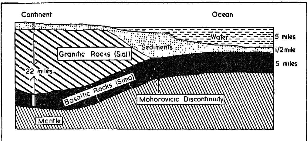
Fig. 13. Profile of the earth's crust
