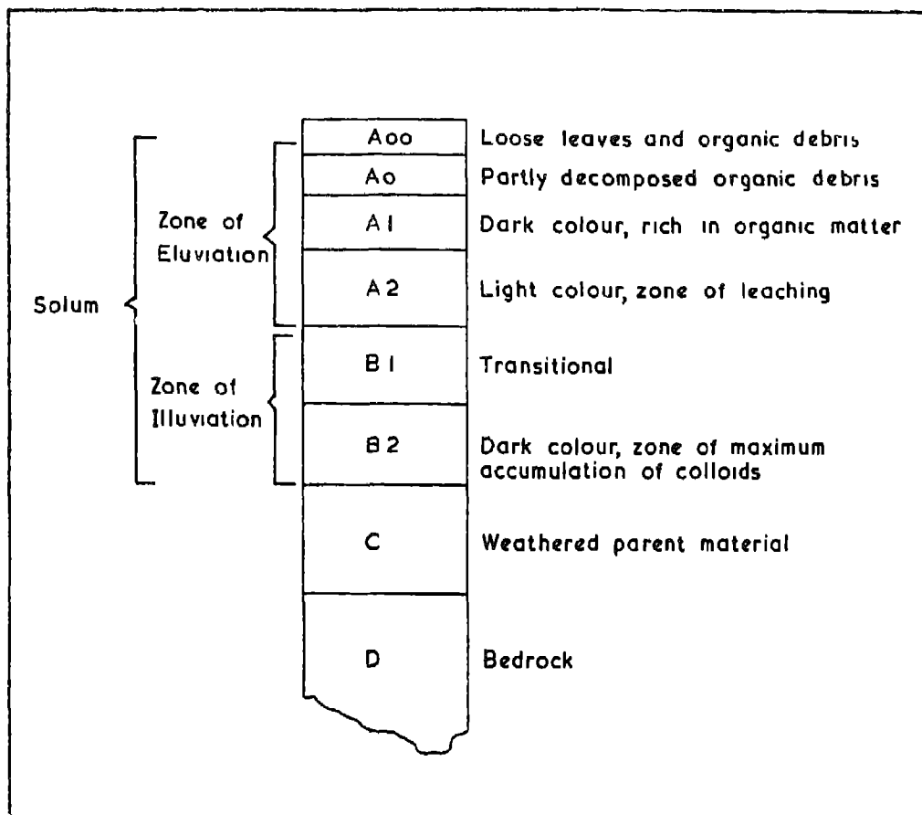
Fig. 21. Generalised Soil Profile
