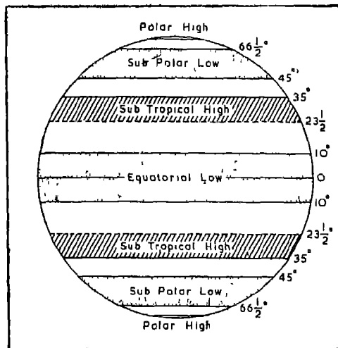
Fig. 68. Pressure Belts
