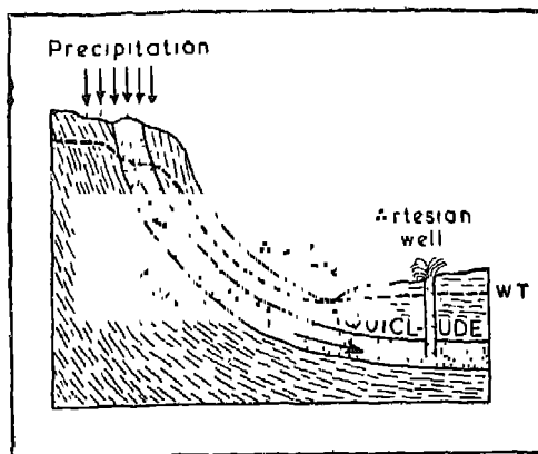
Fig. 93. Geological conditions for Artesian flow
