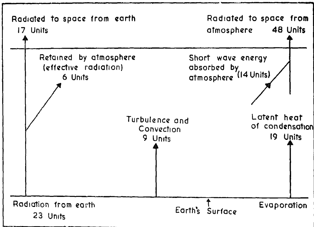
Fig. 61. Terrestrial Radiation
