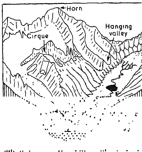
Fig. 41. Glacial Features
