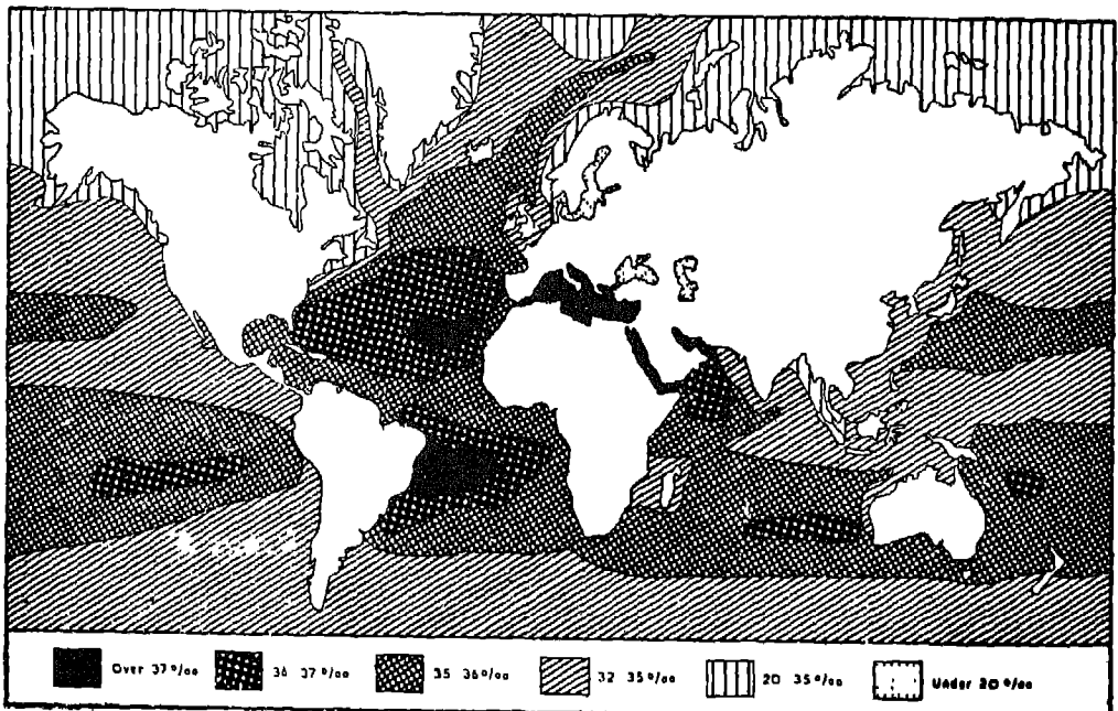
Fig. 103. Distribution of Salinity
