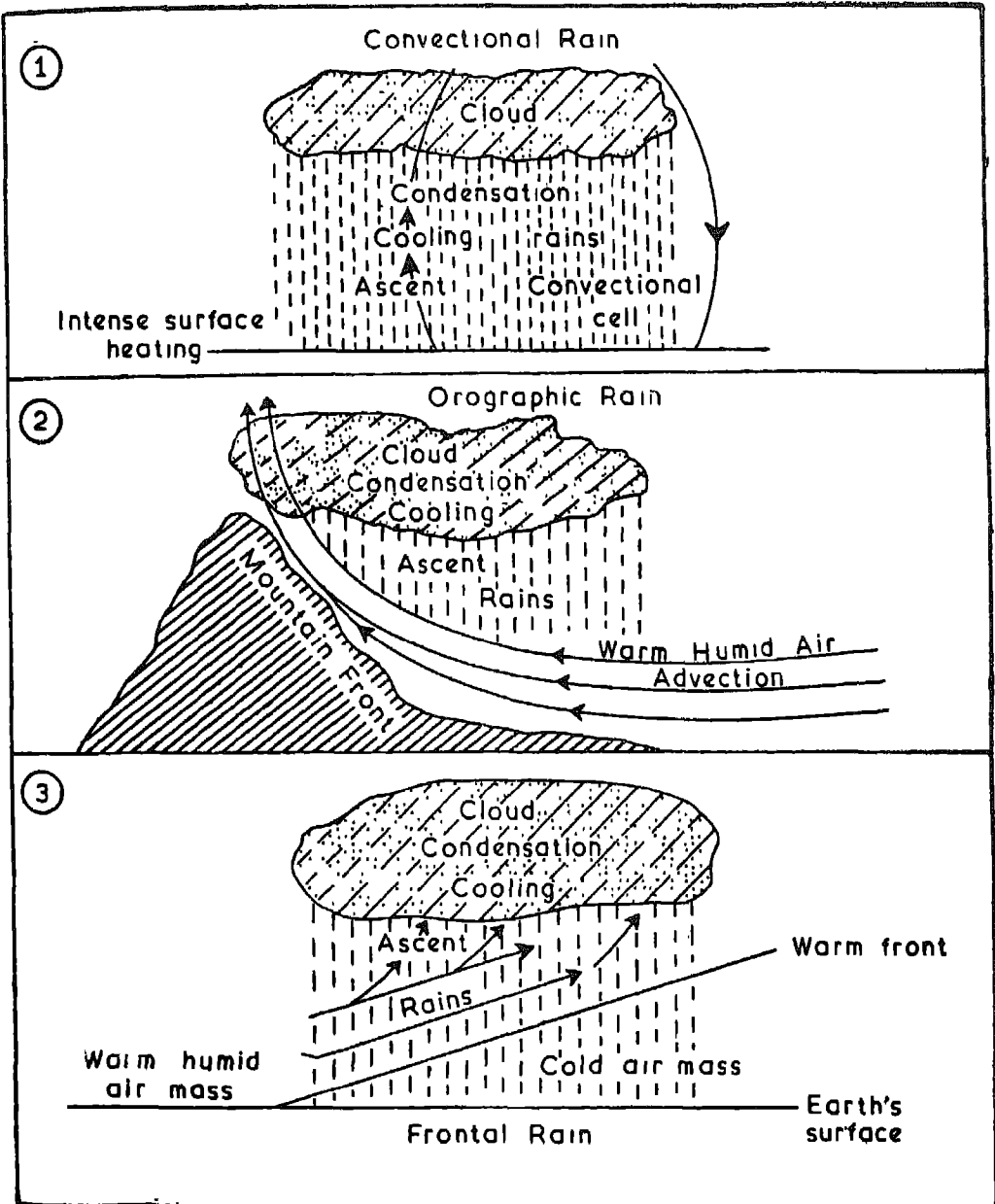
Fig. 78. Convective Rain, Orographic Rain and Frontal Rain
