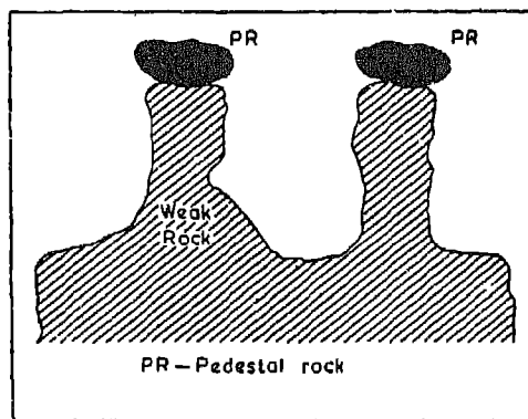
Fig. 39. Pedestal Rock
