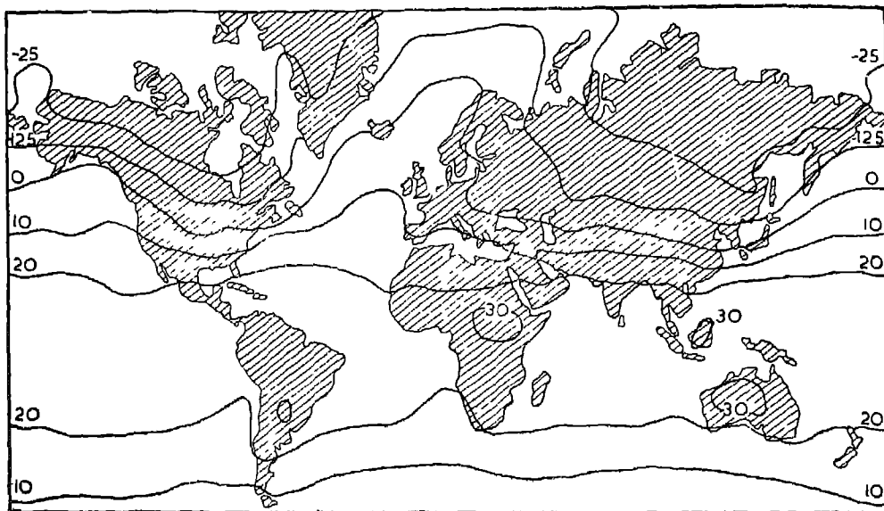
Fig. 63. January Isotherms
