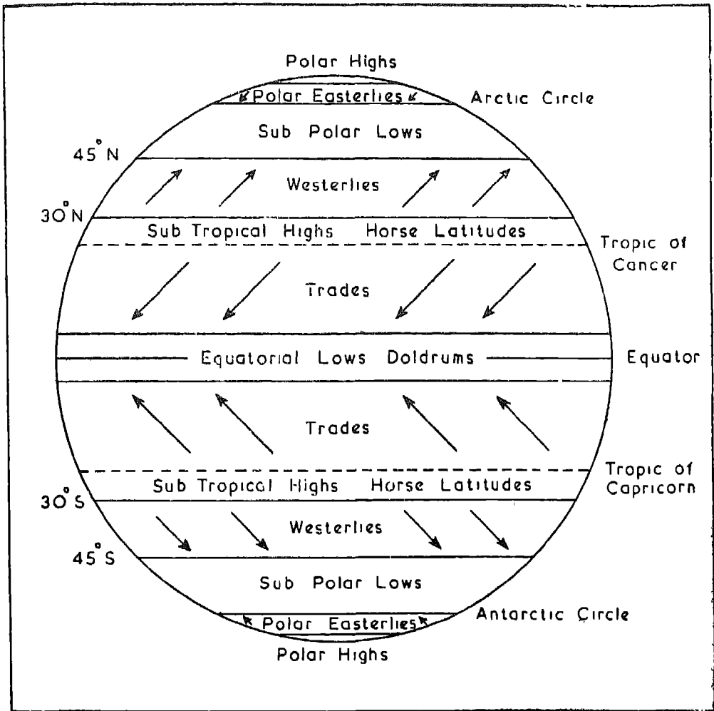
Fig. 70. Planetary Winds
